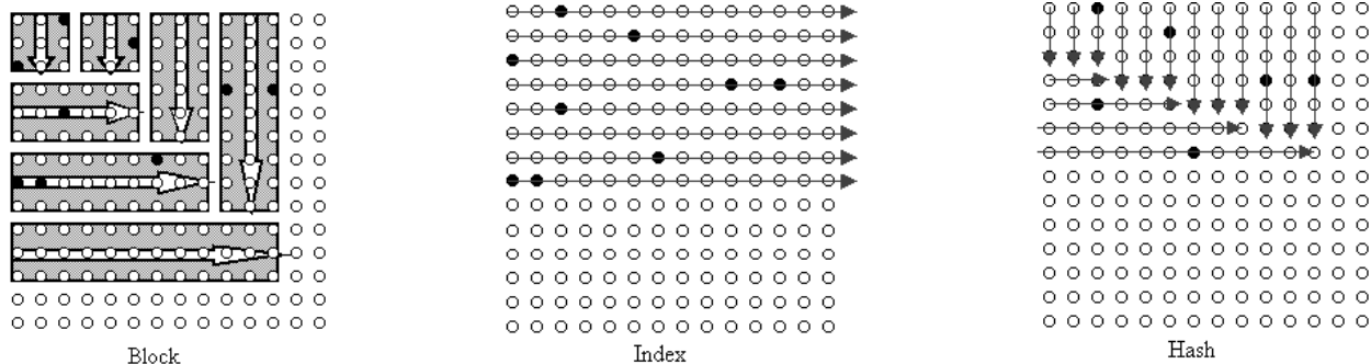
Figure 3: Tuples generated by block, index, and hash ripple join. In block ripple, all tuples are generated by the join, but some may be eliminated by the join predicate. The arrows for index and hash ripple join represent the logical portion of the cross-product space checked so far; these joins only expend work on tuples satisfying the join predicate (black dots). In the hash ripple diagram, one relation arrives 3× faster than the other.
