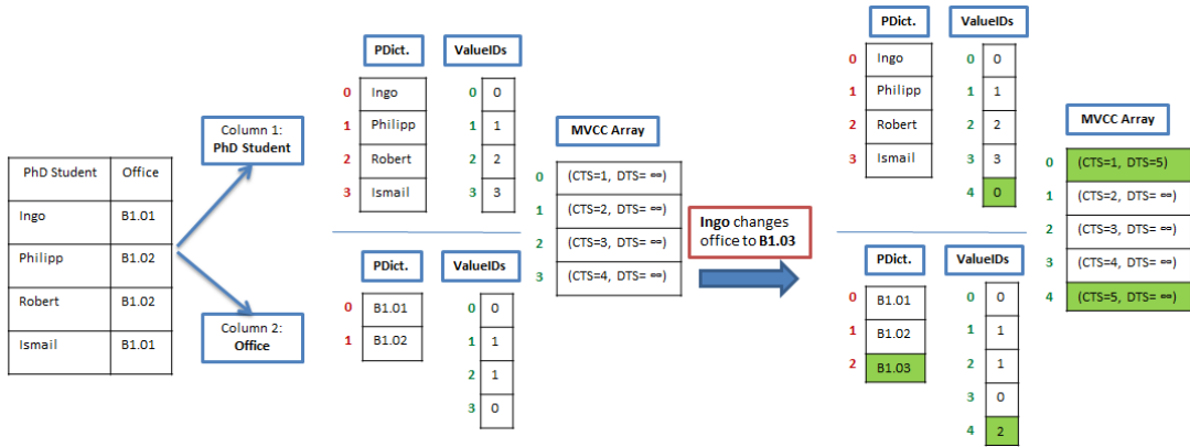
Figure 2: Example of a SOFORT PTable. The office of Ingo is updated from B1.01 to B1.03.
